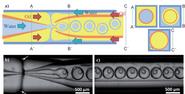
Figure 1. a) Microfluidic capillary device for preparation of W/O/W/O triple emulsion drops. The three cross-sectional schematics (A–A', B–B', and C–C') are included for clarity. b,c) Optical microscope images showing triple emulsion generation and downstream motion. The white arrows in (b) denote the aqueous stream for the outer layers.
